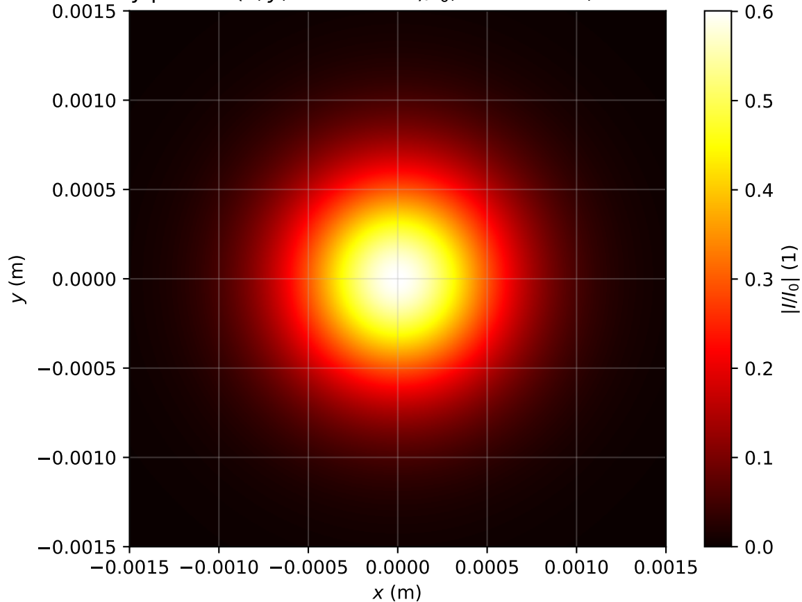
Intensity profile I(x, y, z = 3.344m)/I_0 , \text{Pin}=0.6\text{Pcr} , artificial time
